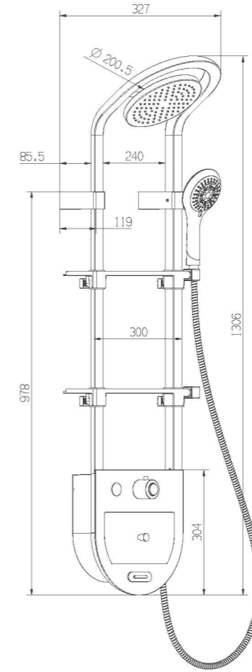
HL-2491 Material: Brass, Aluminum, and ABS Size: 350x280x1306mm Hand Shower: 5F8002
